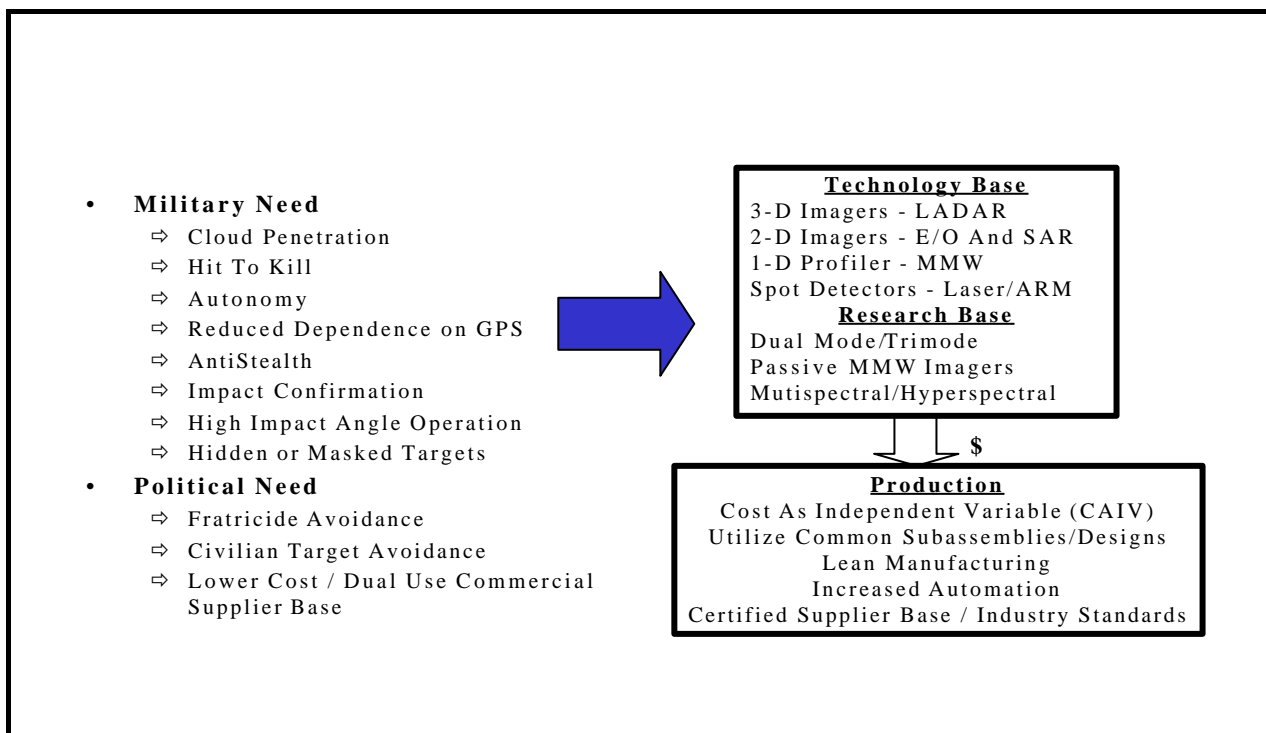
Figure 4. Future Investments
