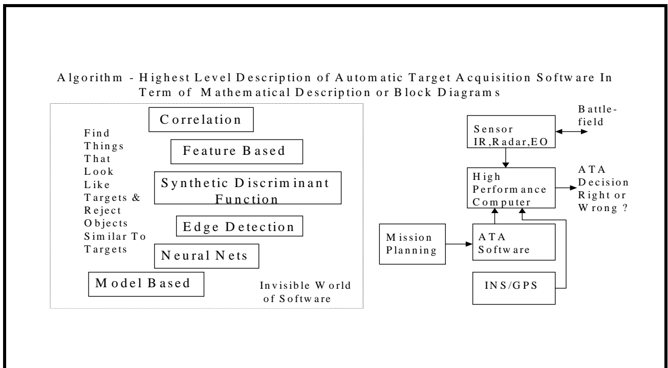
Figure 3. ATR Algorithms
