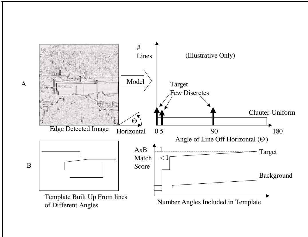
Figure 10. Template Complexity
