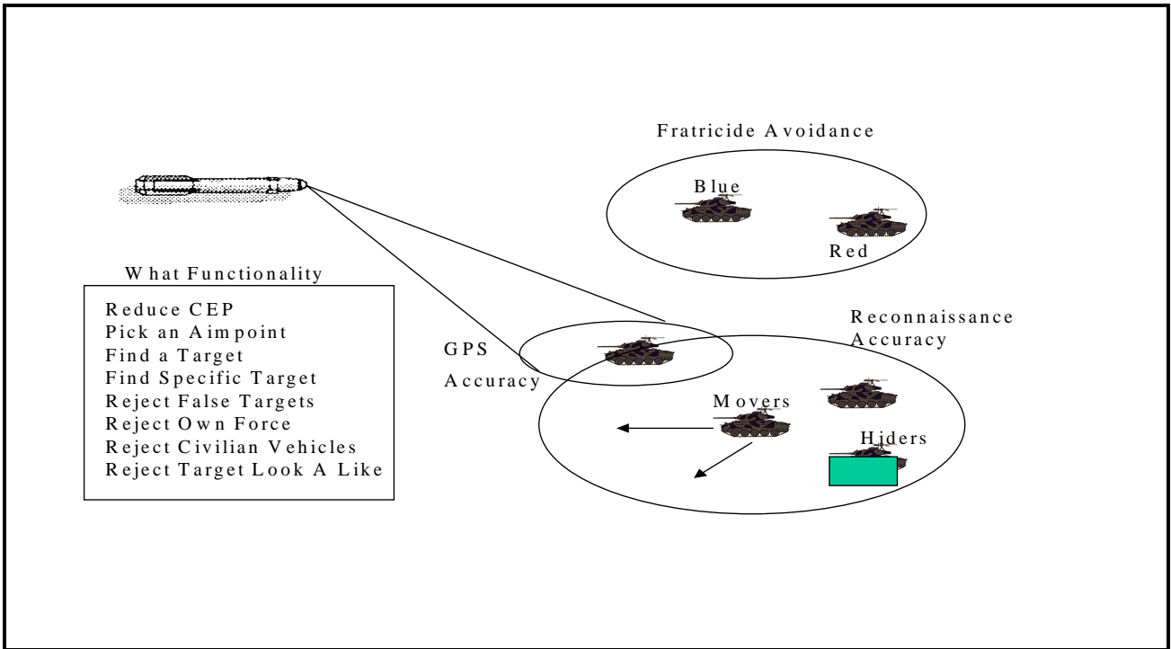
Figure 14. Armor Target
